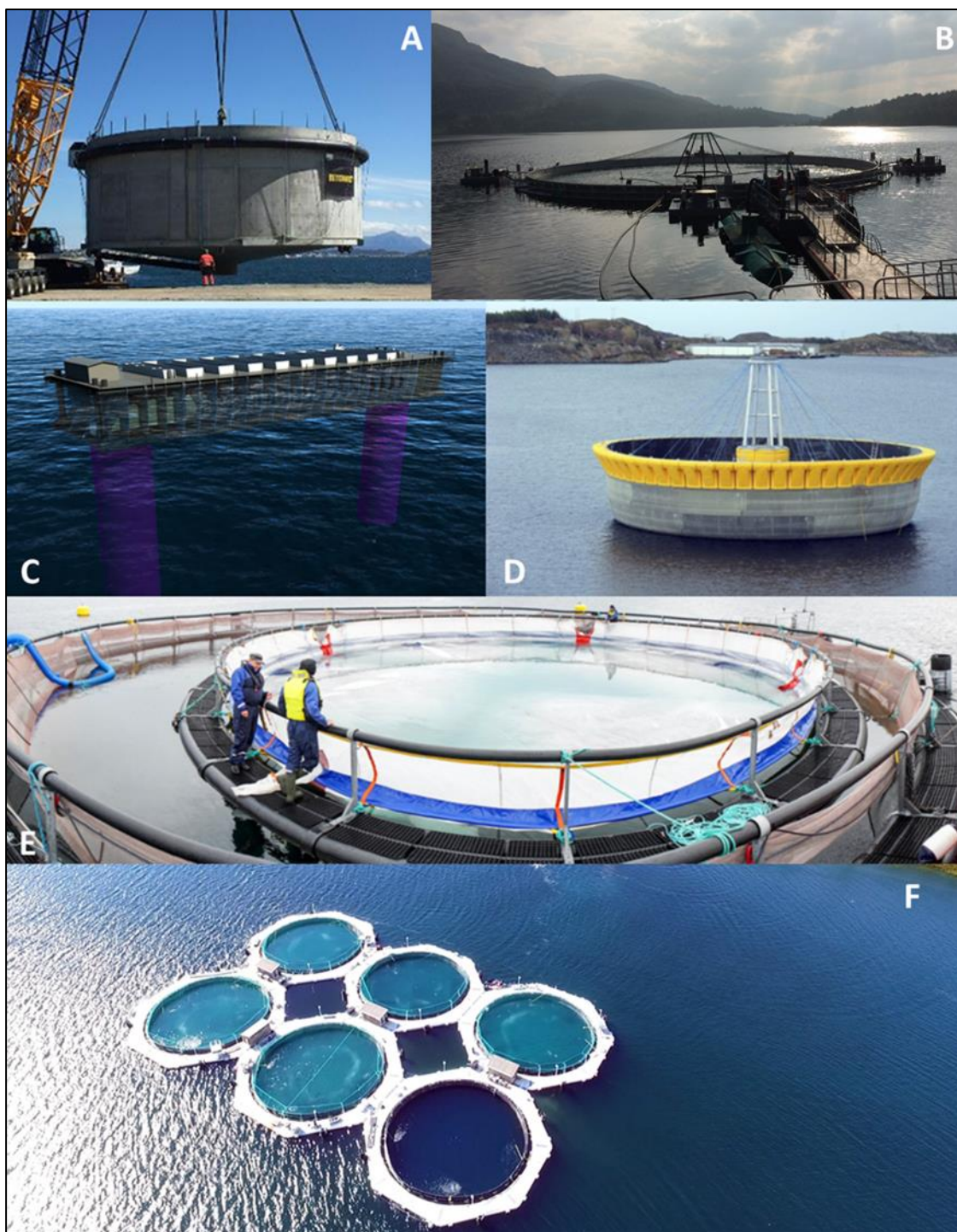
Figure 6.1-1. Different type of semi-closed systems in the sea: A) “Salmon Home #1” concrete tank (photo: Jelena Kolarevic, Nofima); B) Neptun (photo: Aquafarm Equipment); C) Preline (photo: Lerøy); D) AgriMarine (photo: Per Gunnar Kvenseth); E) FlexiBag (photo: Nekton havbruk AS); F) AquaDesign (photo: AquaDesign AS). Photo C) is reproduced with permission from Klemet Steen, Lerøy, photos D) and E) are reproduced with permission from Maria Sørøy, Smøla Klekkeri og Settefiskanlegg AS and photo F) is reproduced with permission from Anders Næss, AquaDesign AS.
