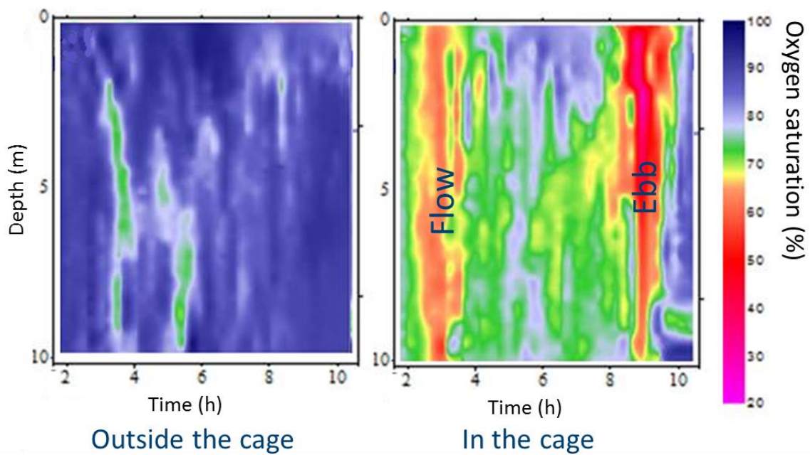
Figure 3.2-2. Example of hypoxic conditions inside a sea cage at slack water. Illustration adapted from [93].
