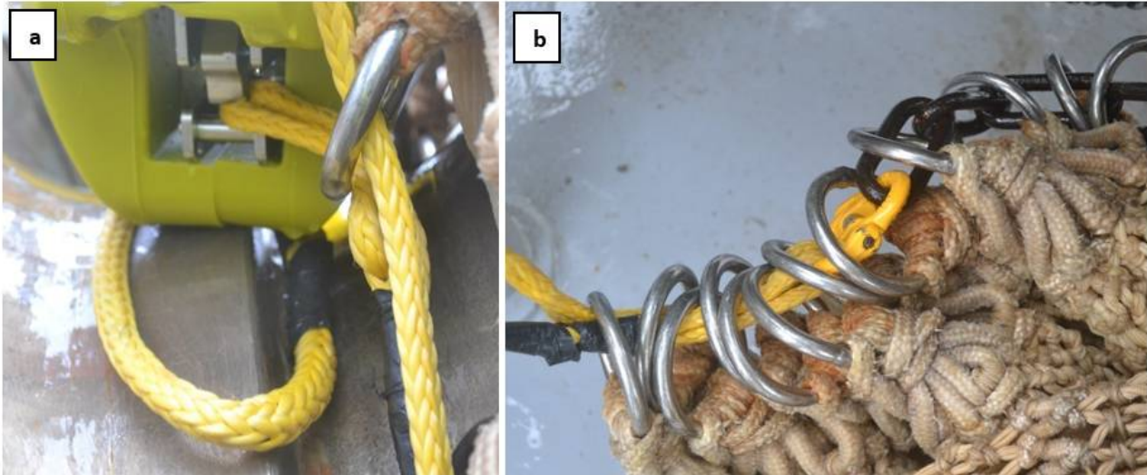
Figure 7.5 – Observations after test C-2 (rig 2); a: the soft eye was only partially released from the releaser jaw; and b: the hammerlock linking the Dynaema twine to the securing chain was jammed in the cod-end skirt rings.
