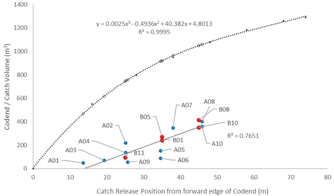
Figure 5.5 - The relationship between the position of the Catch Limit Releaser (CCU) and the resultant cod-end and catch volumes. Theoretical (third order polynomial; R^2 0.9995) cod-end volume estimates are shown in black, and theoretical volume calculated specifically for each haul as open grey diamonds. The resultant catch volume (m 3 ) for each haul is shown for cruise 1 (blue) and cruise 2 (red), with a combine fitted linear relationship (black solid line; R^2 0.7651).
