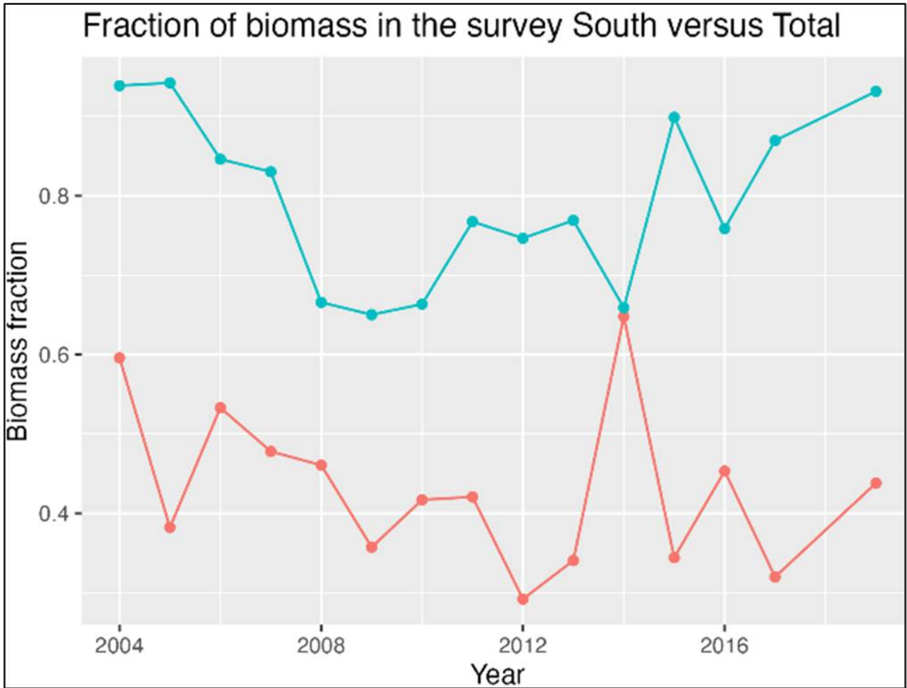
Figure 9.8.1b Fraction of the biomass of cod (red) and haddock (blue) in the southern strata. Most years (2004-2019, no data 2018) > 50% of the biomass of cod is to the north. NB poor coverage in 2014 in the north due to ice.
