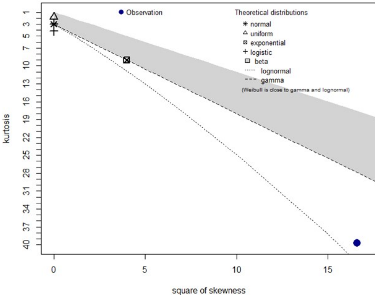
Figure 9.3.5. Visualization of the WP2 biomass dataset with respect to kurtosis and skewness, and in relation to several well-known statistical distributions
