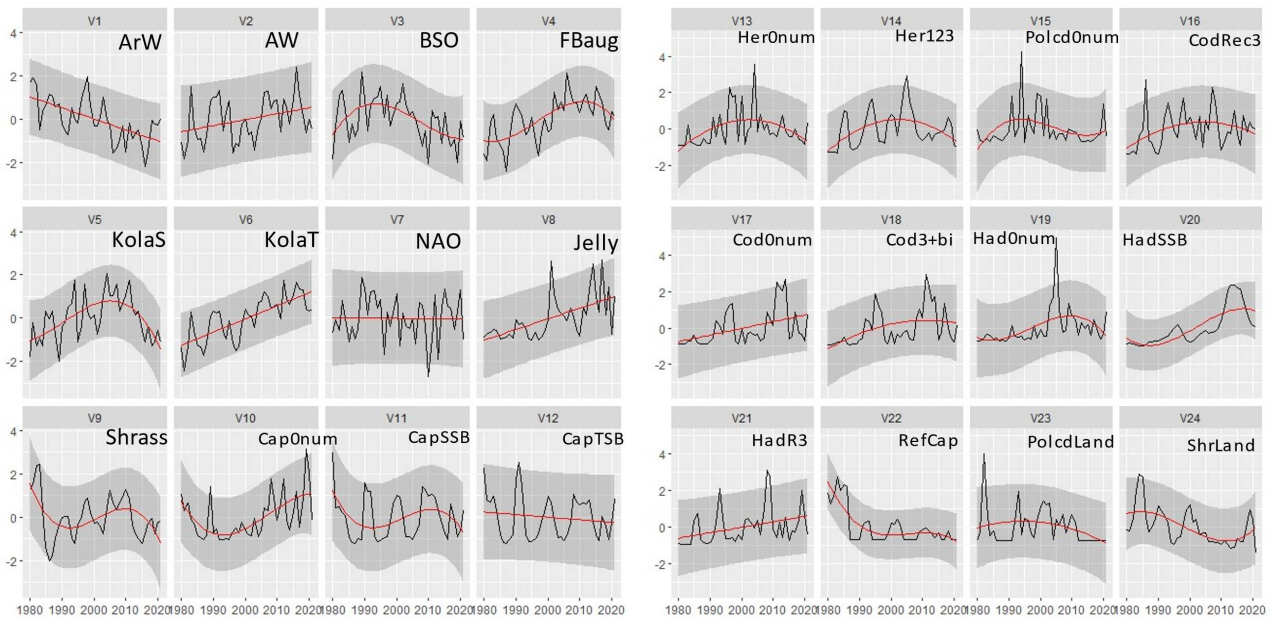
Figure 9.13.1. Time series data observed 1980-2021 applying trend analysis at WGIBAR 2021. Black: observation; Red: Estimated trend; Grey band: Uncertainty trend.
