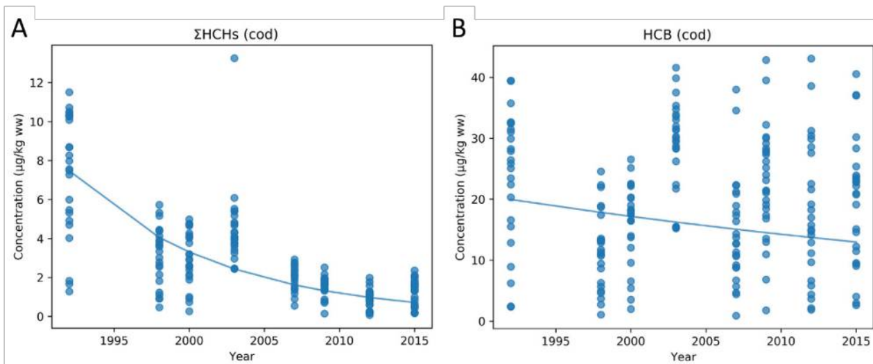
Figure 9.2.2. The levels of chlorinated POPs in cod liver for all individuals (the dots), in \mu\text{g}/\text{kg} wet weight, and the regression model corrected for the median fish weight (the curve), in the period 1992 – 2015. A: sum of alpha-, beta- and gamma-hexachlorocyclohexane ( \Sigma\text{HCHs} ); B: hexachlorobenzene (HCB). From Boitsov et al., 2019.
