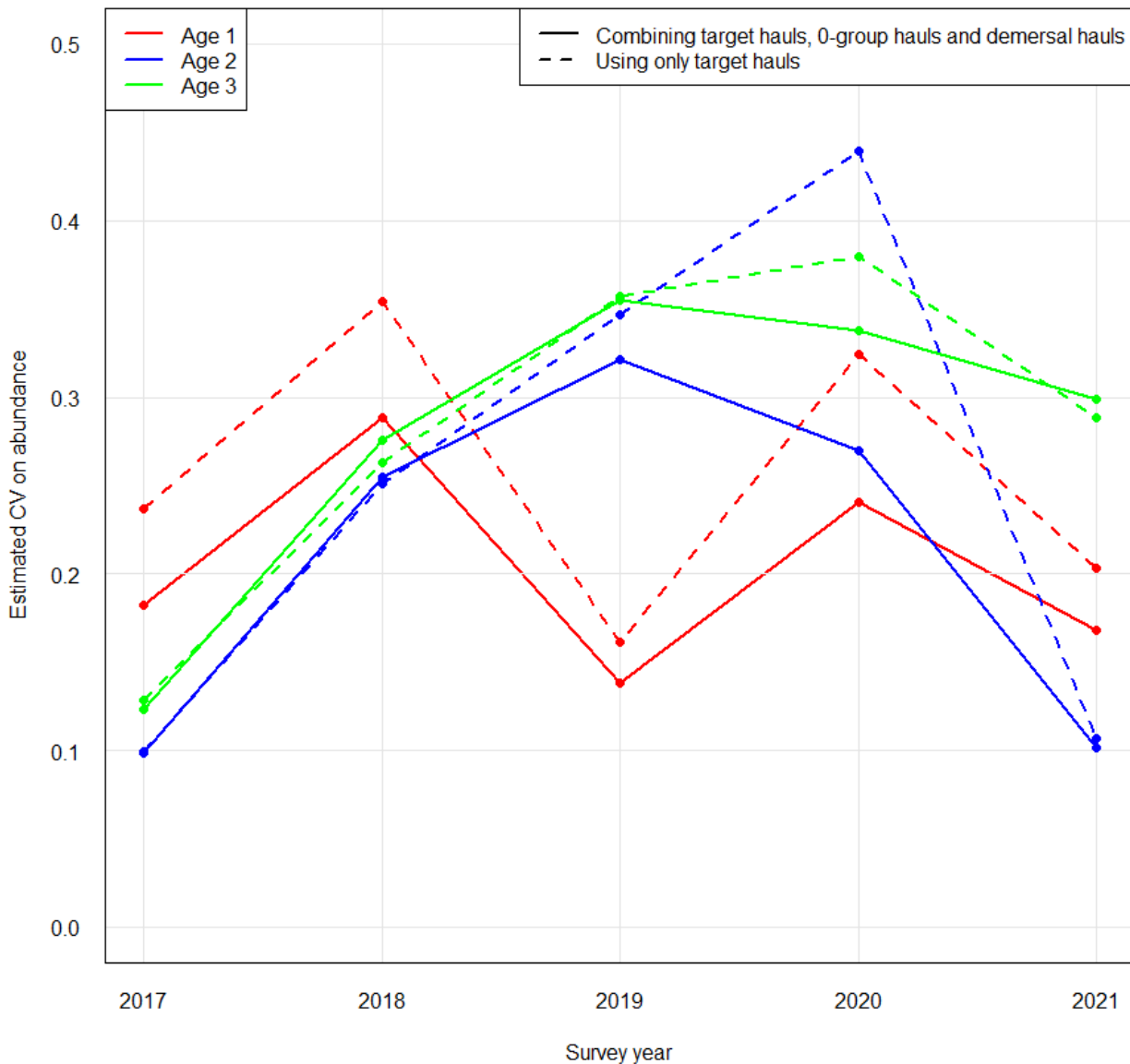
Figure 9.6.2. CV on capelin abundance by age for 2017-2021 comparing estimates based on two different trawl datasets: 1) using a combination of target hauls, 0-group hauls and demersal hauls (used in original assessment; fully drawn lines), and 2) using only target hauls (dashed lines).
