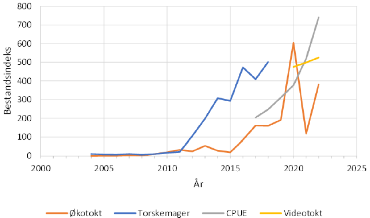
Figure 9.11.1. Stock index based on BESS, findings of snow crab in cod stomachs, CPUE from the fishery and data from the video-observations.
