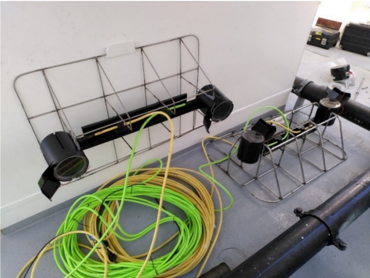
Figure 7: Stereo camera systems rigged prior to deployment on the side panels of the transfer channel.
